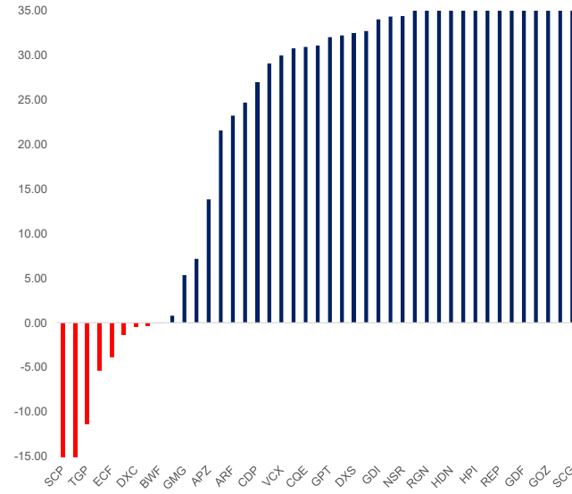
Gearing (%)
